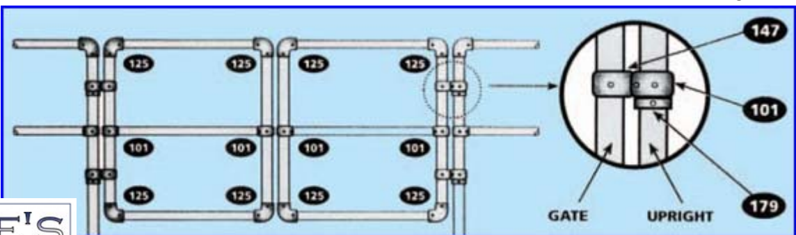
B, C & D sizes 33.7, 42.4 & 48.3mm dia galvanised tube available in 3.25m & 6.5m lengths
